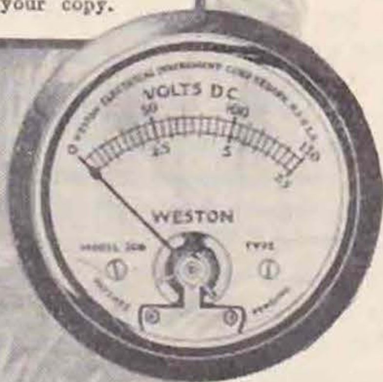
Model 506.—Panel Voltmeters ensure permanent accuracy. With a high internal resistance of 125 ohms per volt, they make practically no load on the batteries. Neat and compact. Prices: £1 15 0 £2 15 0
