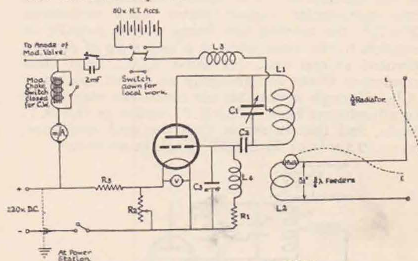
28 MC. TRANSMITTER AT EI7C.
